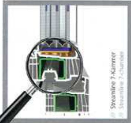
/// Große Stahlarmierung /// Large steel reinforcement
